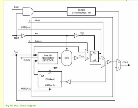
Fig 10. PLL block diagram
