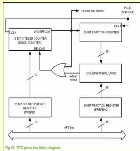
Fig 57. RTC prescaler block diagram
