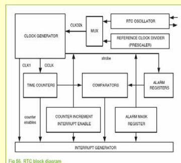
Fig 56. RTC block diagram
